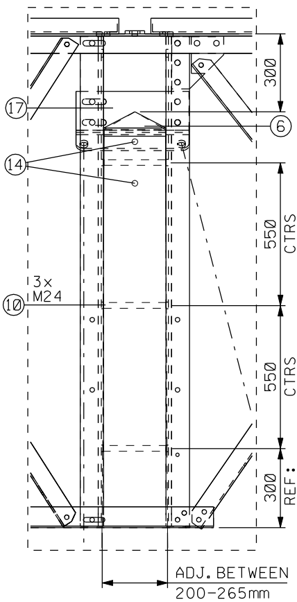
ENLARGED DETAIL 'A'
